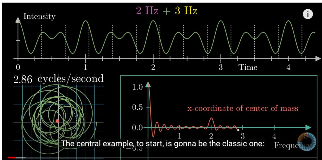
Figure 1 Fourier Transform
